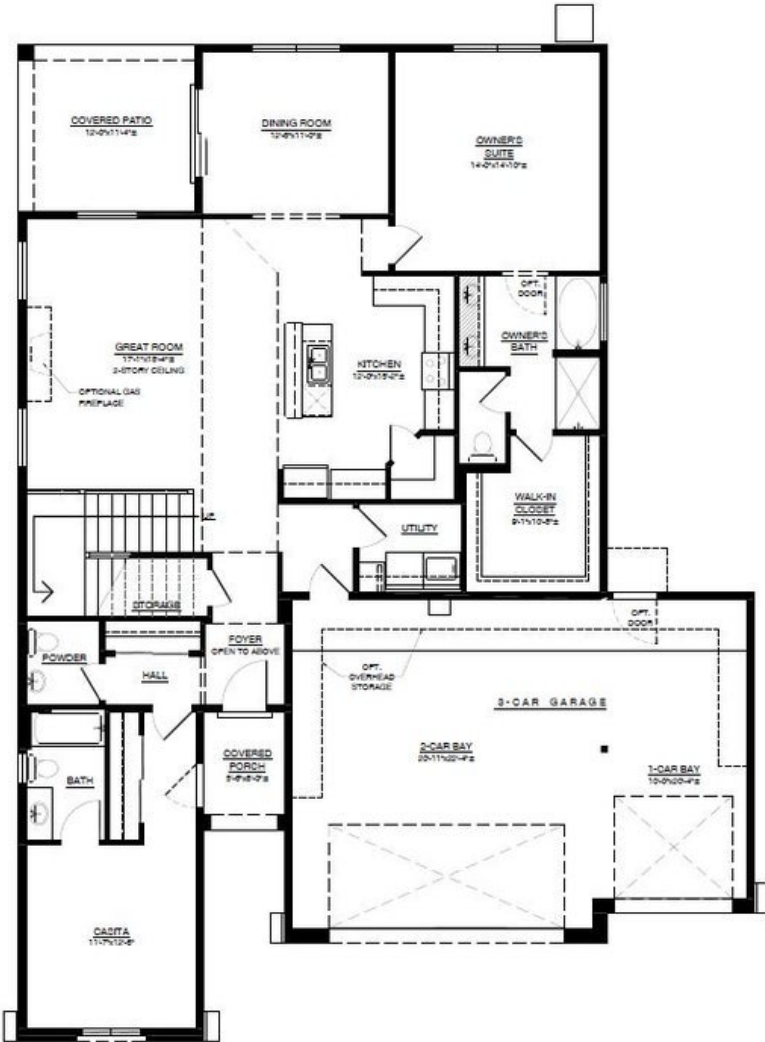
FIRST FLOOR W/OPT. CASITA & OPT. 3-CAR GARAGE
