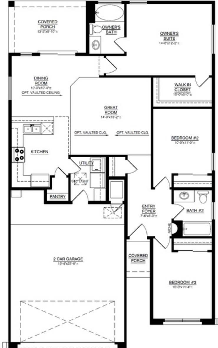
FLOOR PLAN
