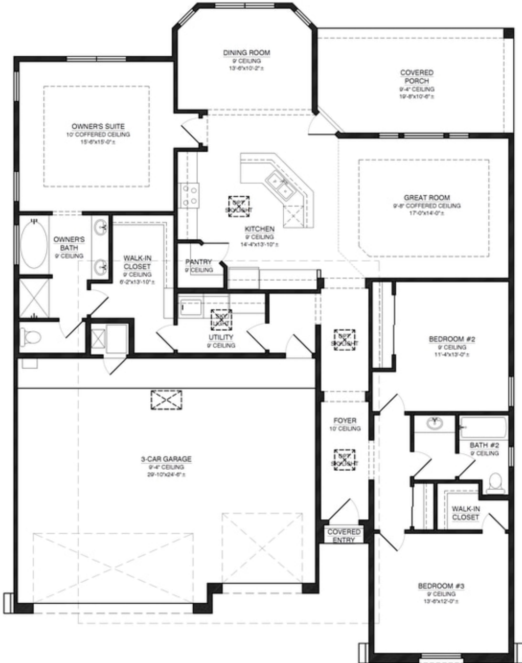
FLOOR PLAN
