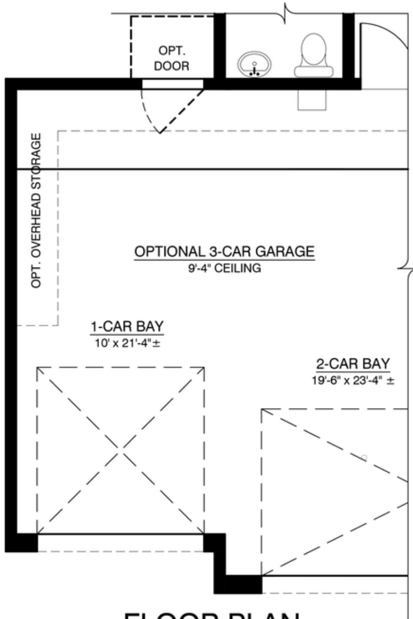
FLOOR PLAN OPTIONAL 3-CAR GARAGE
